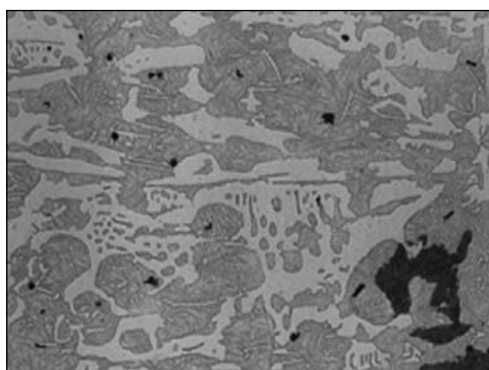
Microstructure MICRA.
